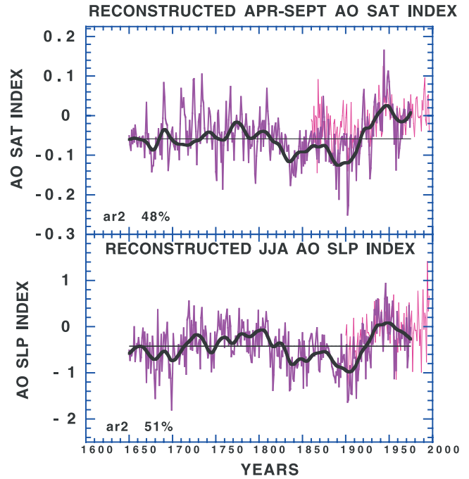
Figure 3. Top: Reconstruction of warm season AO SAT index for AD 1650–1975; annual (purple) and smoothed (black) lines. Red line is instrumental data; variance has been adjusted to correspond to tree-ring estimates. Mean line also indicated. Bottom: JJA AO SLP index. This model accounts for 51% of the variance and also verifies using several statistical tests (e.g., RE = .14 ).
