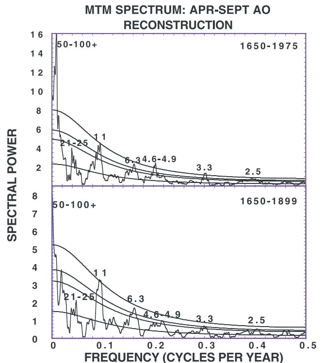
Figure 4. Multi-taper method (MTM) spectral analysis for AO SAT reconstruction. Black lines indicate null, 90%, 95%, and 99% levels of significance. Top: full period from 1650–1975; bottom: 1650–1899.
