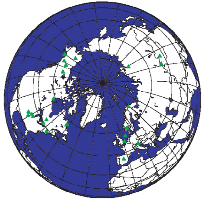
Figure 1. Map showing tree-ring sites (triangles) used to reconstruct the AO SAT index. The sites include Arctic and elevational treeline; and North Atlantic sector locations. Triangles may represent more than one site. Results similar for AO SLP index.
