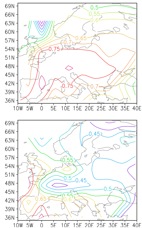
Fig. 5 Correlation over the years 1500–2000 AD between the best pseudo-simulation and the reconstruction of Luterbacher et al. (2004) in winter (DJF, top) and in summer (JJA, bottom) for a 10-year averaging period
