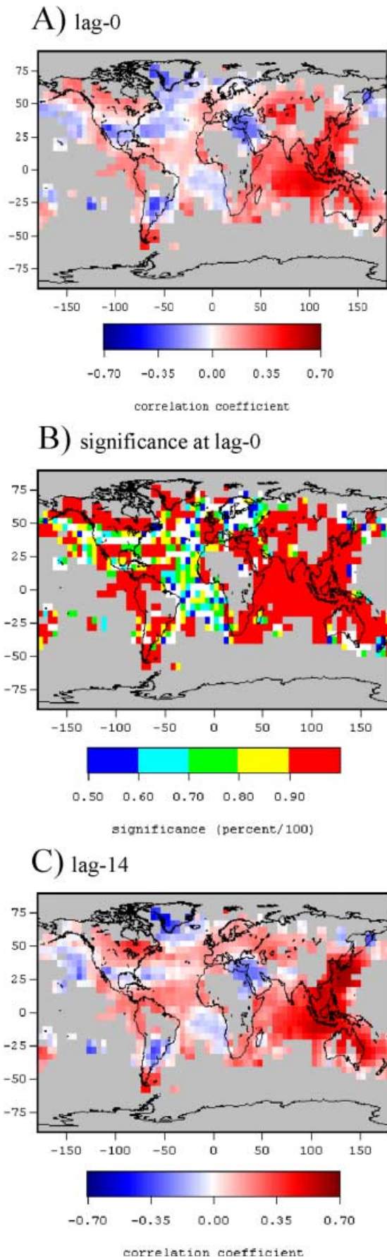
Fig. 2A–C. Correlation pattern between Mann et al. (1998) proxy-reconstructed surface temperature patterns and Lean et al. (1995) solar irradiance reconstruction for the period 1650-1850. Significance levels are shown at the 50-60% level (dark blue), 60-70% level (cyan), 70-80% in green, 80-90% in yellow and and > 90% (red) based on a two-sided test taking into account serial correlation. Shown are both correlation patterns for lag=0 and correlation pattern for lag=14 corresponding to maximum global-mean correlation. Missing data is masked with a gray background
