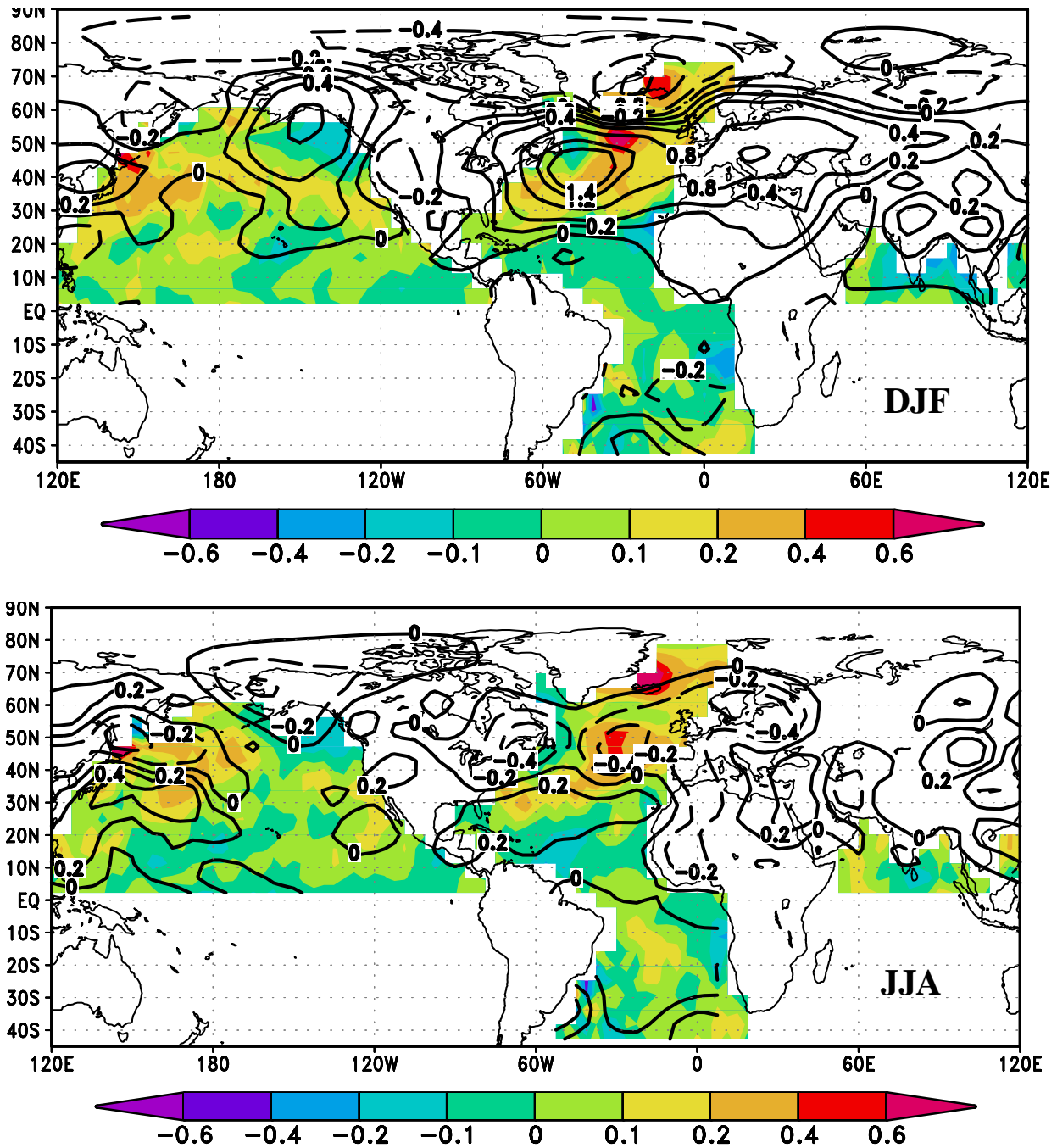
Fig. 6 Spatial pattern of multidecadal signal in model SST and SLP fields based on seasonal mean analyses (same domain of analysis as described for Fig. 5). The phase shown corresponds approximately to phase 90 from Fig. 5.
