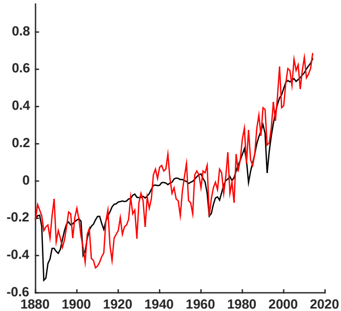
Global Mean GISTEMP vs CMIP5-all forcing
