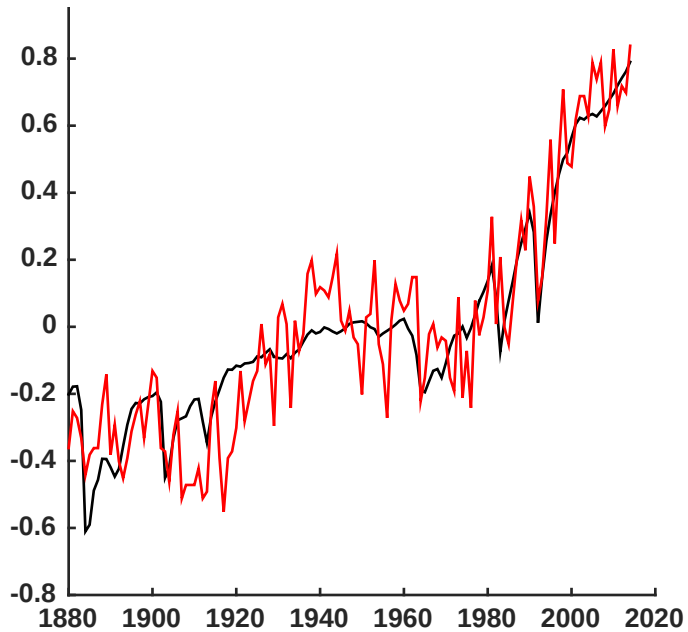
NH Mean GISTEMP vs CMIP5-all forcing
