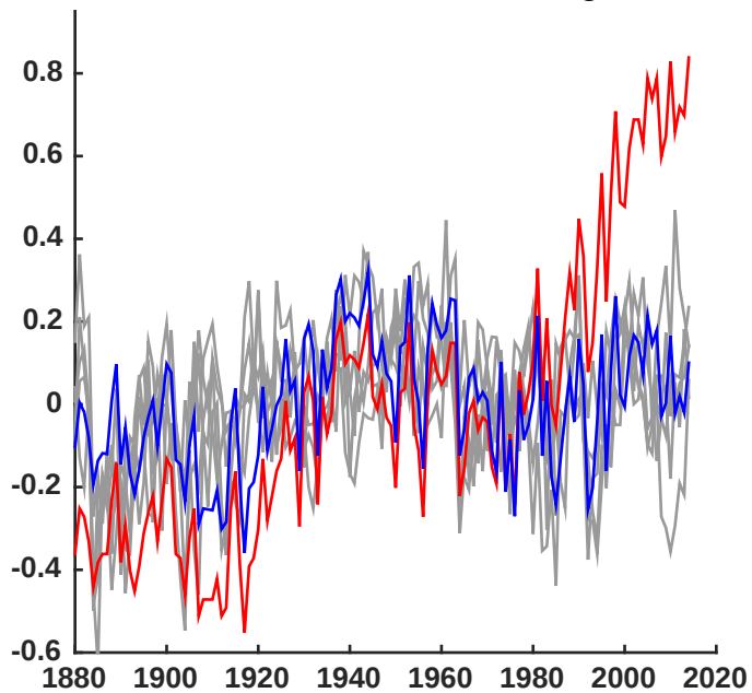
NH Mean CMIP5-all forcing
