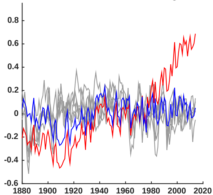
Global Mean CMIP5-all forcing
