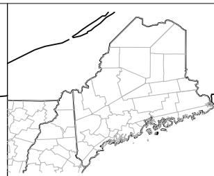
5: MODERATE SNOW
