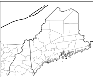
2: SNOW SHOWER
