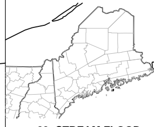
23: STREAM FLOOD
