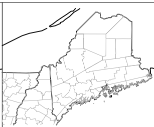
3: SNOW SQUALL
