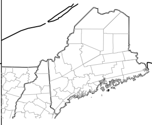
14: BLOWING DUST
