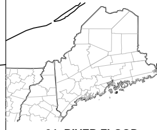
24: RIVER FLOOD
