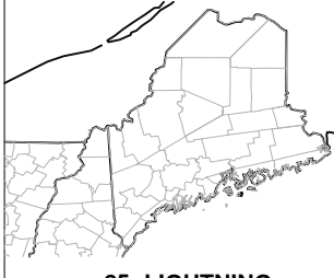
25: LIGHTNING
