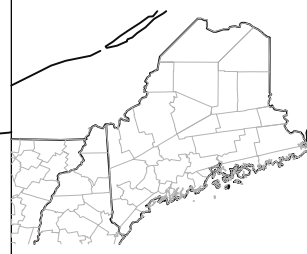
12: HIGH WINDS
