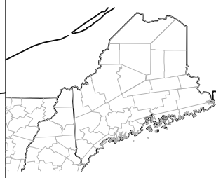
10: SLEET
