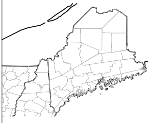
13: SEVERE WINDS
