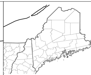
6: HEAVY SNOW
