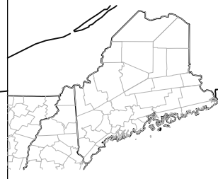
17: DENSE FOG
