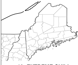
19: EXTREME CHILL
