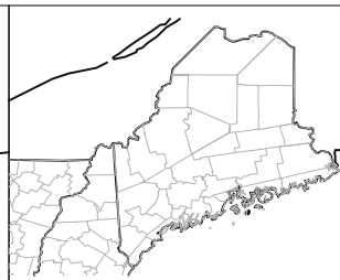
4: LIGHT SNOW
