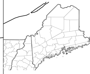
18: WIND CHILL
