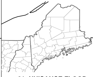
21: NUISANCE FLOOD
