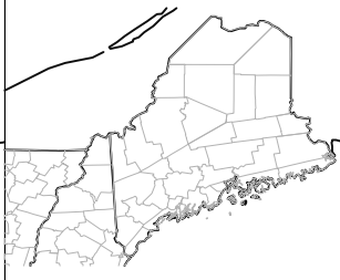
15: BLOWING SNOW
