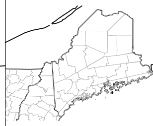
11: ICE STORM
